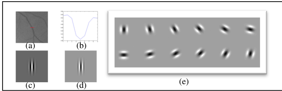
Figure 1: Showing the characteristics of vessel boundaries, the symmetric Gabor kernel and the Gabor filter bank. (a) is a panel cropped from a gray-level retinal image; (b) a gray level profile from the red line crossing the vessel in (a); (c) Gabor kernel with parameter \varphi=0 ; (d) Gabor kernel with parameter \varphi=\pi ; (e) is optimized Gabor filter bank for retinal vessel feature extraction.
