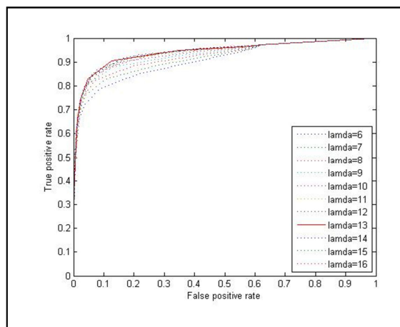
Figure 2: the ROC curves obtained by different lambda values.
