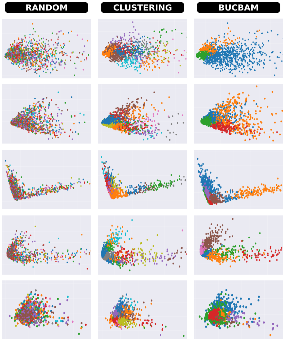
Figure 5: Illustration of the projection of the samples of the clusters on their two first principal components (obtain by PCA) for the three different methods: random split (left) clustering with Kmeans, K=16 (middle) and our BUCBAM proposal (right). In each graph, each color represents a certain cluster. For all the methods, each line represents the instances of a specific category, that is the same than the one represented at the same line in Figure 4. Note that, in contrast to other methods, ours provide clusters with different amount of colors for each specific category. Best view in PDF.
