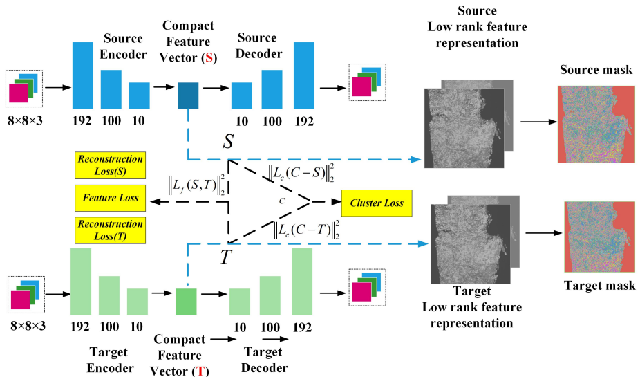
Figure 3: Overview of our DCAE architecture. S and T represent the encoded representation of the source and target images respectively. C represents the cluster centroid closest to T. The triangle depicts how our losses are calculated.
