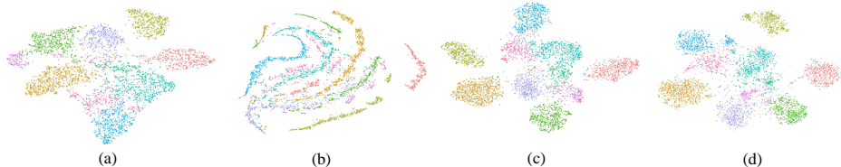
Figure 2: t-SNE visualization on AWA with Attribute semantic on (a) SOC [28], (b) SSE [14], (c) JLSE [14], and (d) ours. Comparing (c) and (d), although both JLSE and our method result in well-separated clusters for each class, each cluster in (d) is more compact and thus improved performance can be expected (see Table 2).
