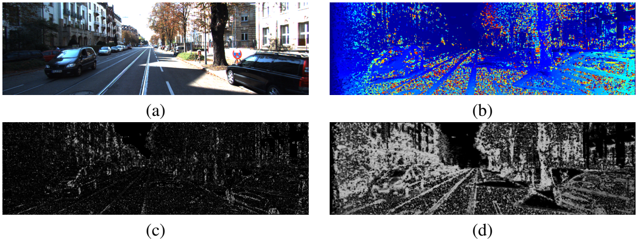
Figure 1: An image from KITTI 2015 dataset. (a) reference image, (b) disparity map (c) confidence map according to Left-Right Difference [14] CM (d) confidence map according to the proposed CCNN.
