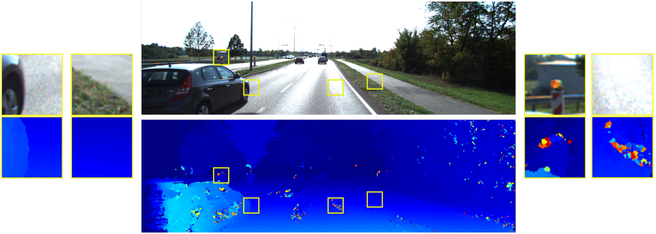
Figure 2: Reference image and disparity map computed by the SGM [11] algorithm with highlighted four regions. On the left, two regions including correct disparity assignments and, on the right, two regions including wrong disparity assignments.
