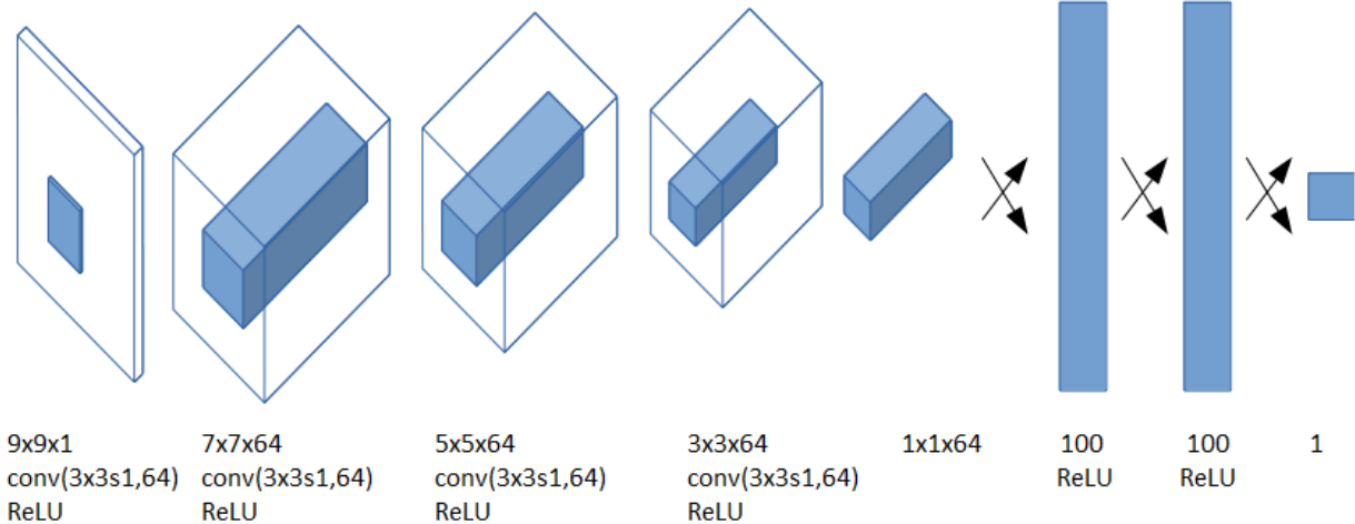
Figure 3: Architecture of the proposed CNN to infer the CM from from the raw disparity map. It is a single channel network, designed for 9 \times 9 image patches. Four convolutional layers apply 64 overlapping kernels (stride equal to 1) of size 3 \times 3 . Two fully-connected layers made of 100 neurons each (i.e., 100 1 \times 1 convolution kernels) lead to the final regression node.
