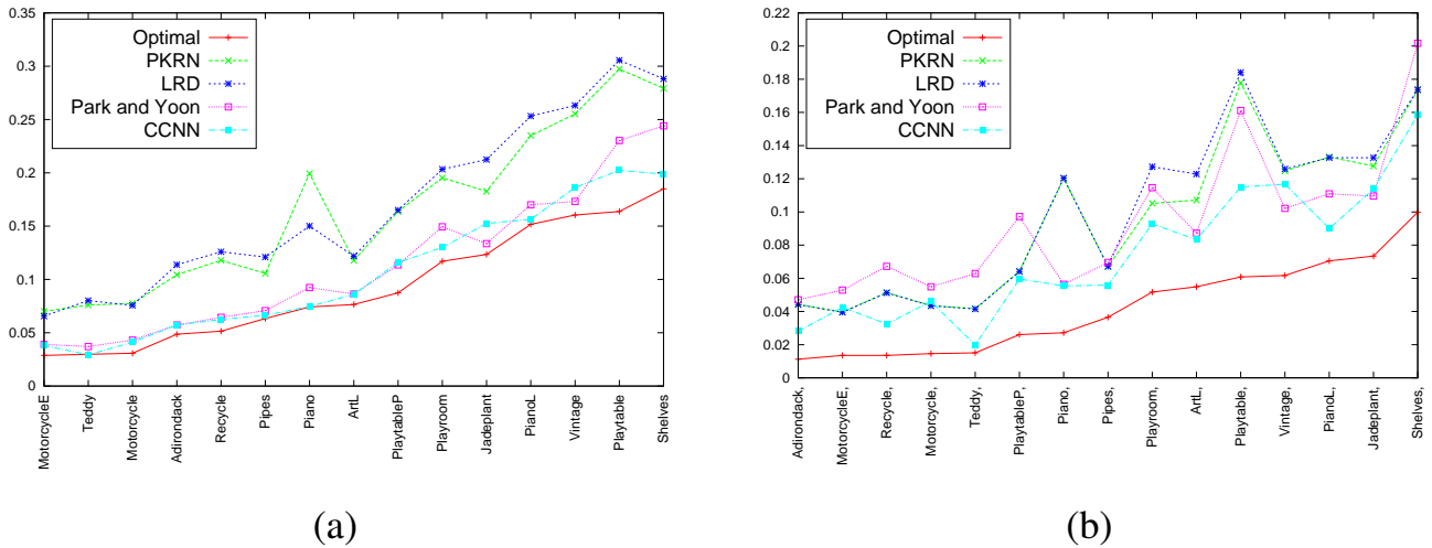
Figure 5: AUC values computed for four CMs (PKRN, LRD, Park & Yoon and proposed CCNN) on Middlebury 2014 dataset sorted in non-decreasing order according to optimal values (in red). The lower, the better. (a) BM algorithm. (b) SGM algorithm.
