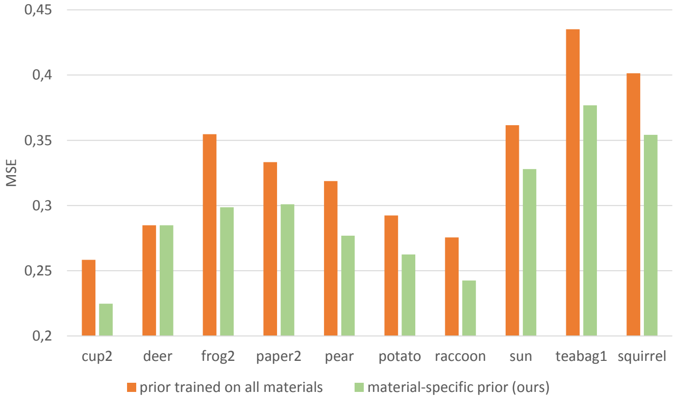
Figure 4: Graph of the error left after optimization. Less is better. Our method of training on specific materials consistently outperforms training on all materials.
