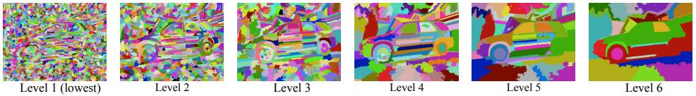
Figure 4: The segments output by SWA at six levels. Note how the segments covering the semantic parts change from level 1 to level 6 (e.g. left windows and left wheels). This illustrates that different parts need different levels of segmentation. For example, the best level for the left-back wheel is level 4 and the best level for the left windows is level 5. Best view in color.
