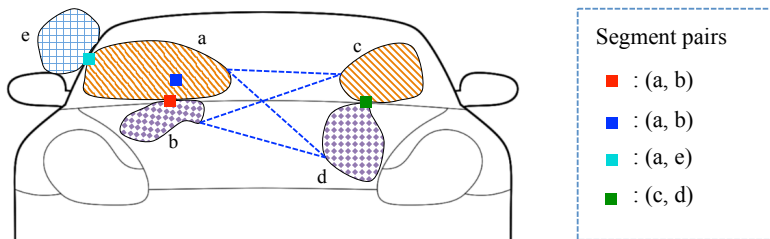
Figure 3: Illustration of segmentation appearance consistency (SAC) and segment pairs. Red and green squares represent two neighboring landmarks lying on the boundary between window and body. Each landmark has two segments ( a and b for the red landmark, c d for the green landmark) close to it. Our method models and learns the SACs for every pair of neighboring landmarks (blue dashed lines) and uses them to enhance the reliability of landmark localization. For the blue landmark, its segment pair is the same as the red landmark, which is the closest one on the boundary.
