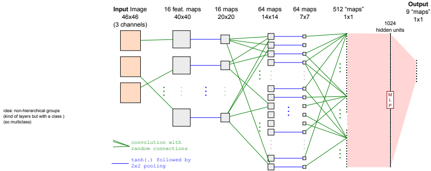
Figure 1: Plain single-scale convolutional architecture presented in [9] for scene labeling
