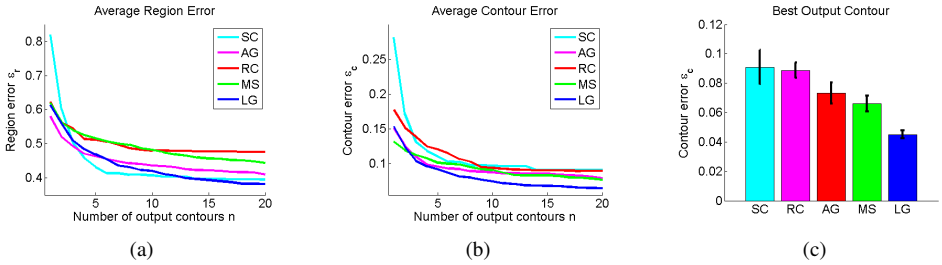
Figure 2: Quantitative evaluation on SOD test dataset. (a) Minimum region error using intersection over union measure as a function of the number of output contours allowed. (b) Minimum contour error using contour mapping measure as a function of the number of output contours allowed. (c) Minimum contour error over all output contours. See Section 6 for a listing of the algorithms tested.
