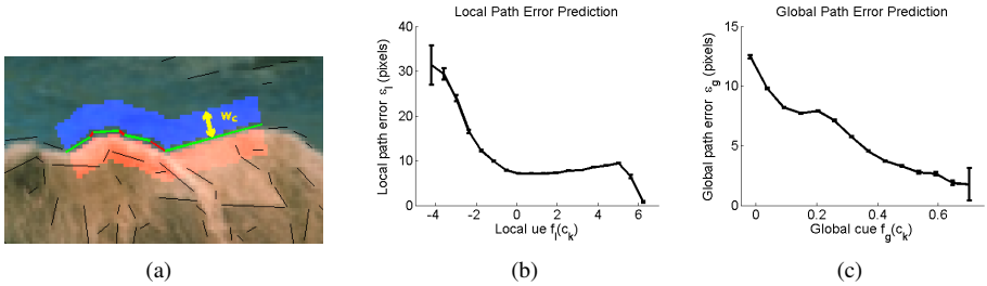
Figure 1: (a) Figure/ground bands used to compute global color contrast cue. (b) and (c) Learned nonparametric predictors for path error based upon local and global cues.
