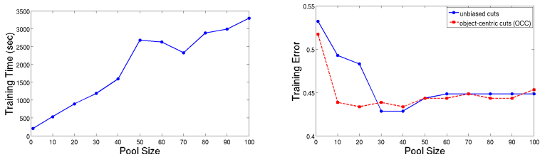
Figure 5: Left: Training time as a function of pool size. Right: Training error as function of pool size, for both uniformly sampled random shifts and the proposed object-centric partitions. By focusing on object-centric shifts, we can achieve a stronger classifier with a smaller total pool, which improves training efficiency.
