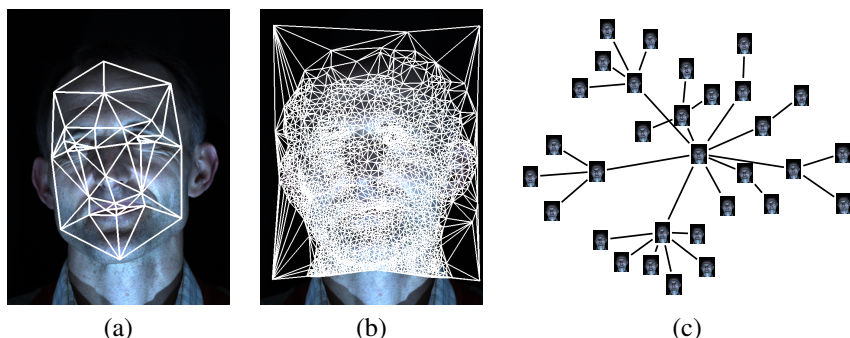
Figure 1: Overview: From a sparse, 37 point AAM (a) the proposed method creates a dense, 1000 point AAM (b) suitable for image synthesis tasks. To achieve the dense registration required to construct the AAM we find a bounded diameter minimum spanning tree on a graph defined on the training images (c). On the digital version it is possible to zoom in to see the individual training images.
