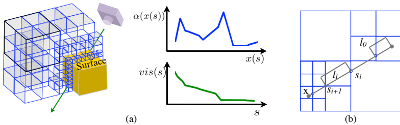
Figure 2: (a) Plots of occlusion density \alpha and vis as a ray travels through volume. \alpha peaks (and visibility drops) as the ray pierces the two outside surfaces of the (almost) hollow yellow cube. (b) A parametrization of the ray into intervals according to octree cell intersections.
