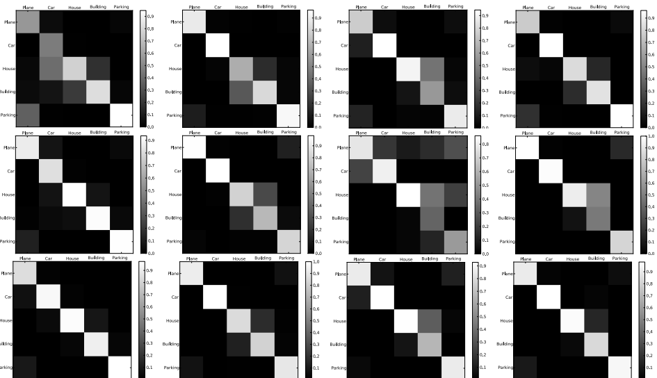
Figure 5: Average confusion matrices (across trials). Columns (left to right): PPFH, SHOT, SI, SC. Rows (top to bottom): Nearest Neighbor, Bayes, SVM. In all cases r_{supp} = 30 and K = 500
