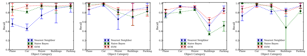
Figure 6: Total recall for all object categories using different classifiers. In all cases, r_{supp} = 30 and K = 500 . From left to right: FPFH, SHOT, SI, SC. Markers correspond to the total recall in all the validation trials. Error bars span the maximum and minimum recall attained by a trial.
