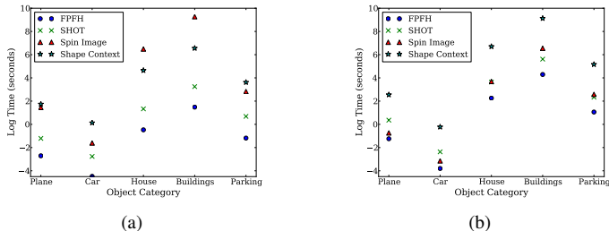
Figure 7: Average running time per object for different descriptors. (a) r_{supp} = 10 , (b) r_{supp} = 45 .
