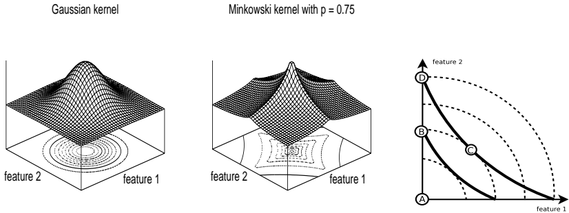
Figure 1: Left: density functions and equidistant contours for the Gaussian kernel. Middle: the proposed Minkowski kernel. Right: the Minkowski kernel is particularly sensitive when multiple feature values change at the same time (point C), whereas the Gaussian is more sensitive to large variations in any one feature (point D).
