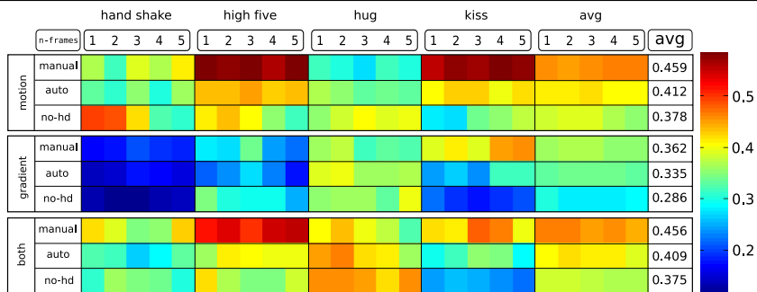
Figure 4: Average classification accuracy results with different parameter combinations. No consistent improvement is noticed by using higher n-frame descriptors. Motion information is a more discriminative feature than gradients in three of the four interactions. On average using head information improves the accuracy. (Best viewed in color).
