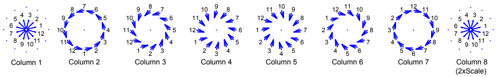
Figure 2: The construction of our 12 \times 8 \mathbf{P} -matrix descriptor. The arrangement is the same as in [2], but we base the descriptor on the 4S-DTCWT. The small numbers (and the orientations of the arrows) denote the subband selected at each sampling location. Each column is composed of a set of rotationally symmetric samples. The figure is taken from [2].
