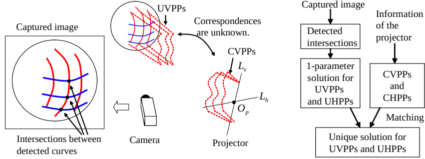
Figure 2: Planes used in the system (left) and the flow chart to estimated the planes (right).
