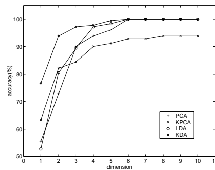
Figure 8: Recognition accuracy.
