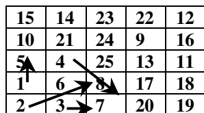
Fig. 1. Displacement vectors for four pixels with the highest ordinal order. The displacement vectors are vectors connecting the locations of pixels with similar gray-level ordinal order in the two compared regions. The sum of the four displacements in this case is 1 + \sqrt{5} + 1 + \sqrt{5} .
