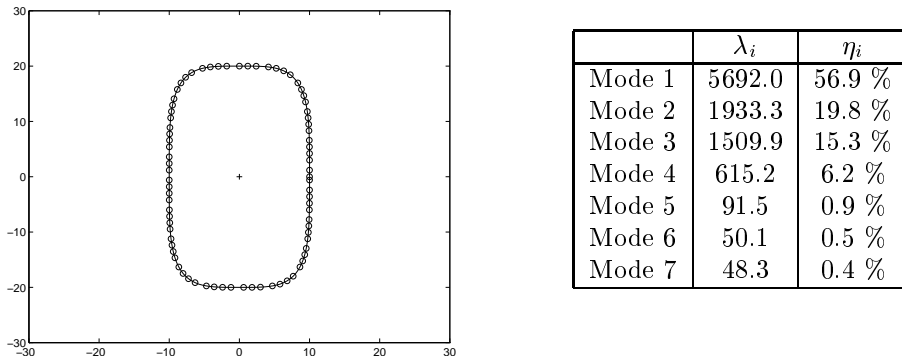
Figure 2: Landmarks of the natural (undeformed) superellipse model (left) and contribution of each mode to the overall point variance over the training set (right).
