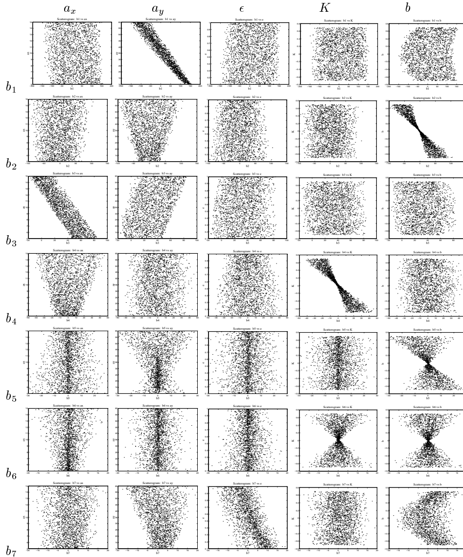
Figure 4: Scattergrams that relates the modes of variation to the original deformable superellipse parameters over the training set. High concentration of points around a line indicate high correlation. It can be seen that modes b_1 , b_2 , b_3 and b_4 , chiefly correlates to a_2 , b , a_1 and K , respectively, and pretty much uncorrelated to other parameters.
