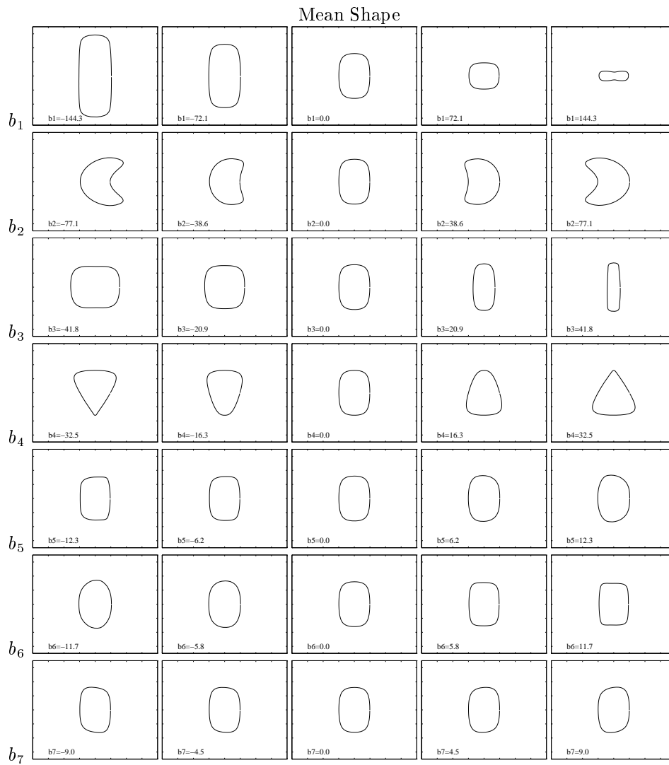
Figure 5: Parametrisation of the PDM model. The modes of variation controls the actual PDM shape in a rather neat way: the first four modes straightly control vertical height, bending, width and tapering, respectively, whereas the last three produce, in combination and unexpectedly, slight horizontal tapering, squaring and shearing.
