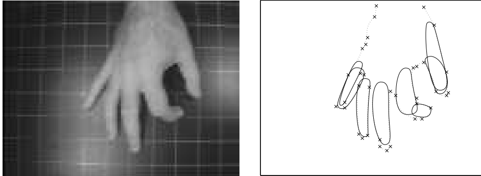
Figure 6: Example of use of the linear superellipse model fitted to some arbitrary object parts. More examples appear in these proceedings in [12]
