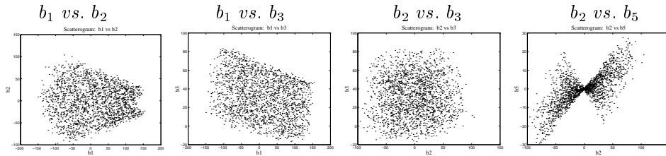
Figure 3: Four examples of scattergrams of the modes of variation. Low-order modes are relatively uncorrelated to each other whereas more and more correlation crops up for higher order modes.
