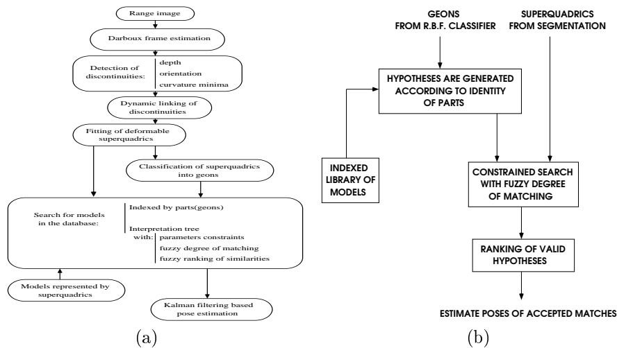
Figure 1: (a) Functional diagram of the complete recognition approach; (b) The matching approach presented here.
