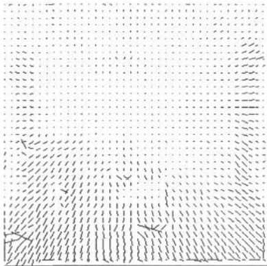
Figure 5.3 The needlemap of the castle sequence. The flow vectors are mostly trained towards the focus of expansion. The flow is meaningful even in part of the hole of the mounting bracket at the lower left side of the image.
