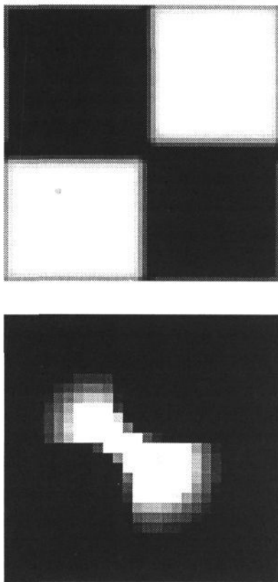
Figure 2.1b The top image controls the width of the filter. The white blocks are areas where the filter should have small support and the black area large support. The point spread function of a bright point placed in the midpoint between the tips of the white squares is shown on the bottom.
