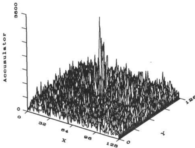
Figure 8. Coherent CHT Accumulator array for a circle image with \sigma_i^2 = 200
