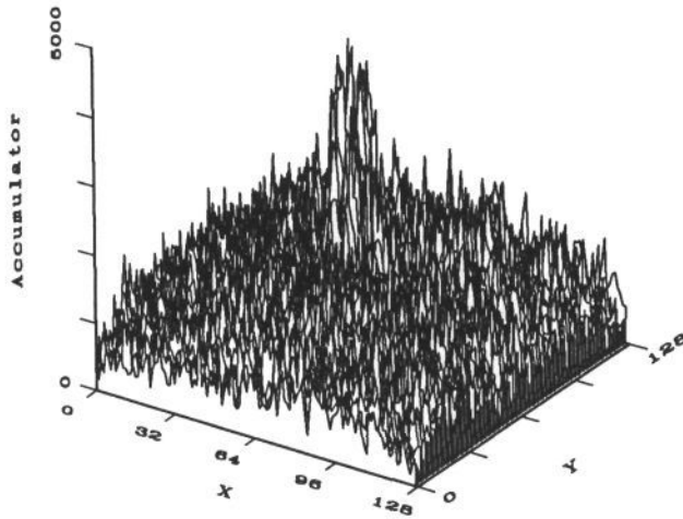
Figure 7. Energy CHT Accumulator array for a circle image with \sigma_i^2 = 200
